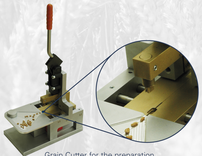
Grain Cutter for the preparation of the grain samples
